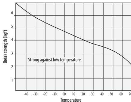
Strength Test: temperature
