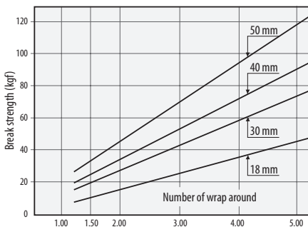
Strength Test: Width and Number of Wraps
