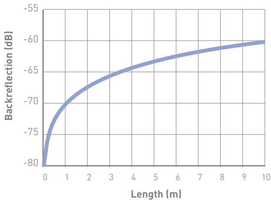
Backreflection VS Length (10m singlemode)
