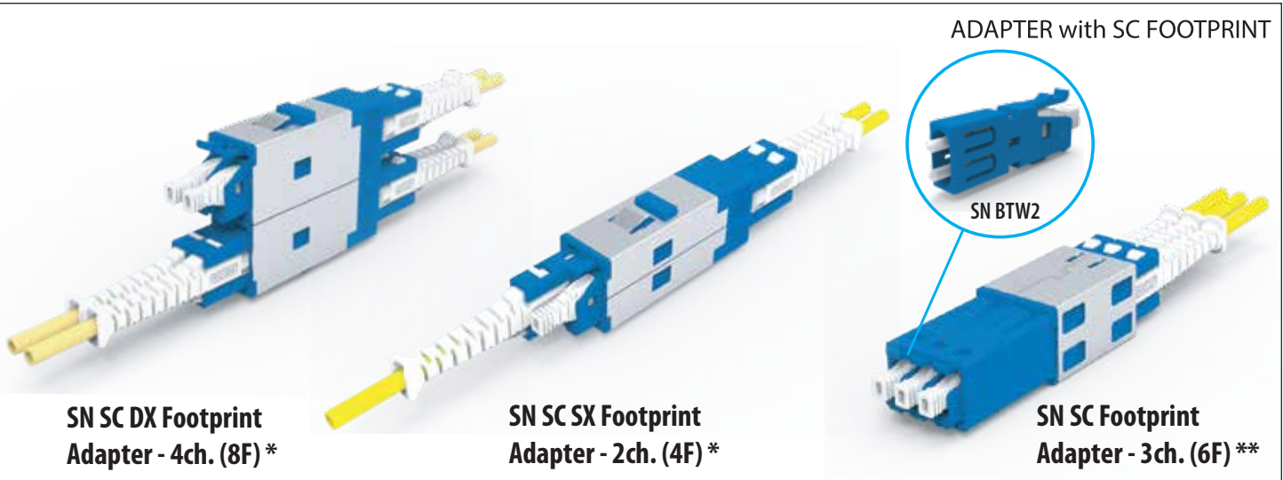
SN Connector 1.6mm boot
