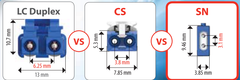
LC Duplex , CS, SN Comparison
