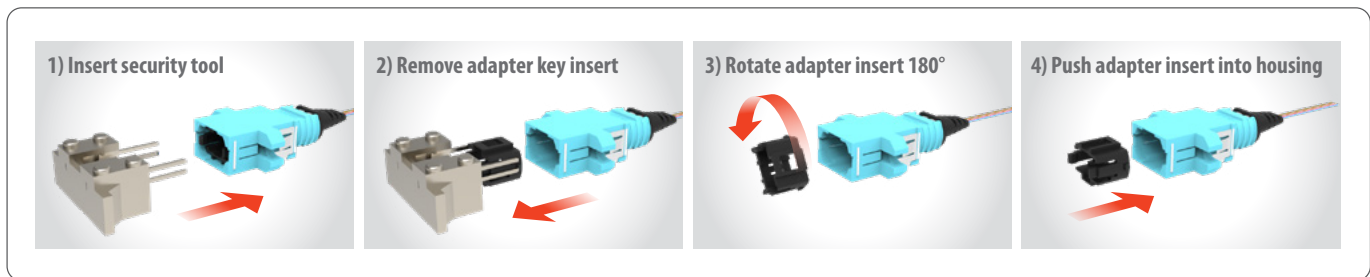
Figure 19 SENKO MPO adapter polarity reversal steps
