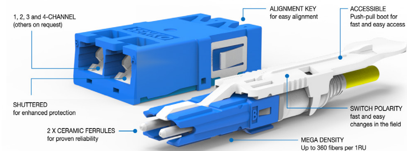
Figure 22 Polarity of SENKO CS® connector is similar to the LC and SC duplex connectors
