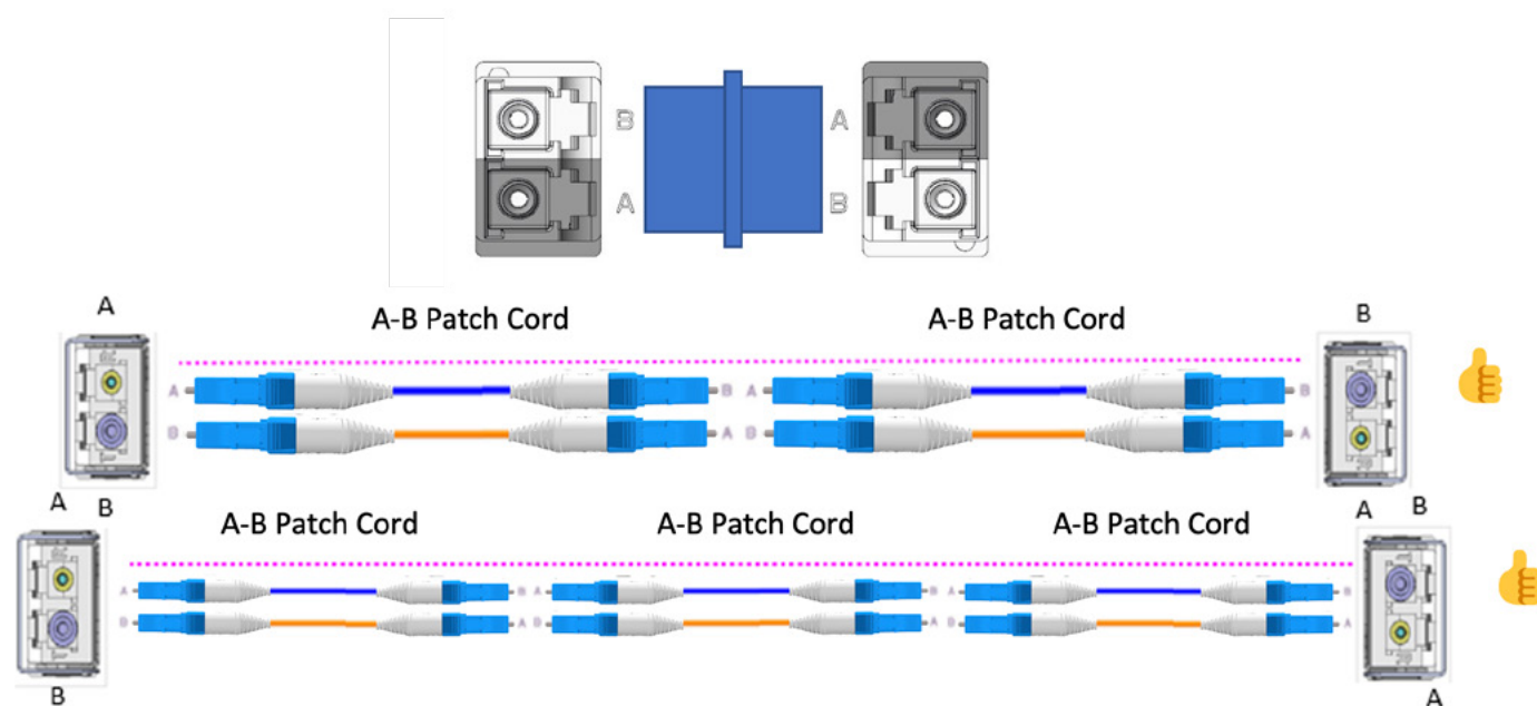
Figure 29 LC Key up to Key up adapter allows any number of A-B patchcords in the system.
