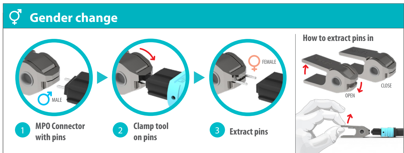
Figure 18 SENKO MPO gender reversal steps
