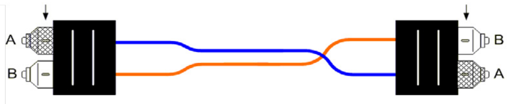
Figure 4 Position A and B configuration of a 568SC
