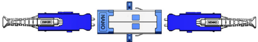
Figure 27 Most common SN® adapter is Key up to Key up.
