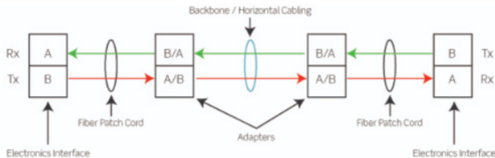
Figure 2 Example of duplex cables interconnection
