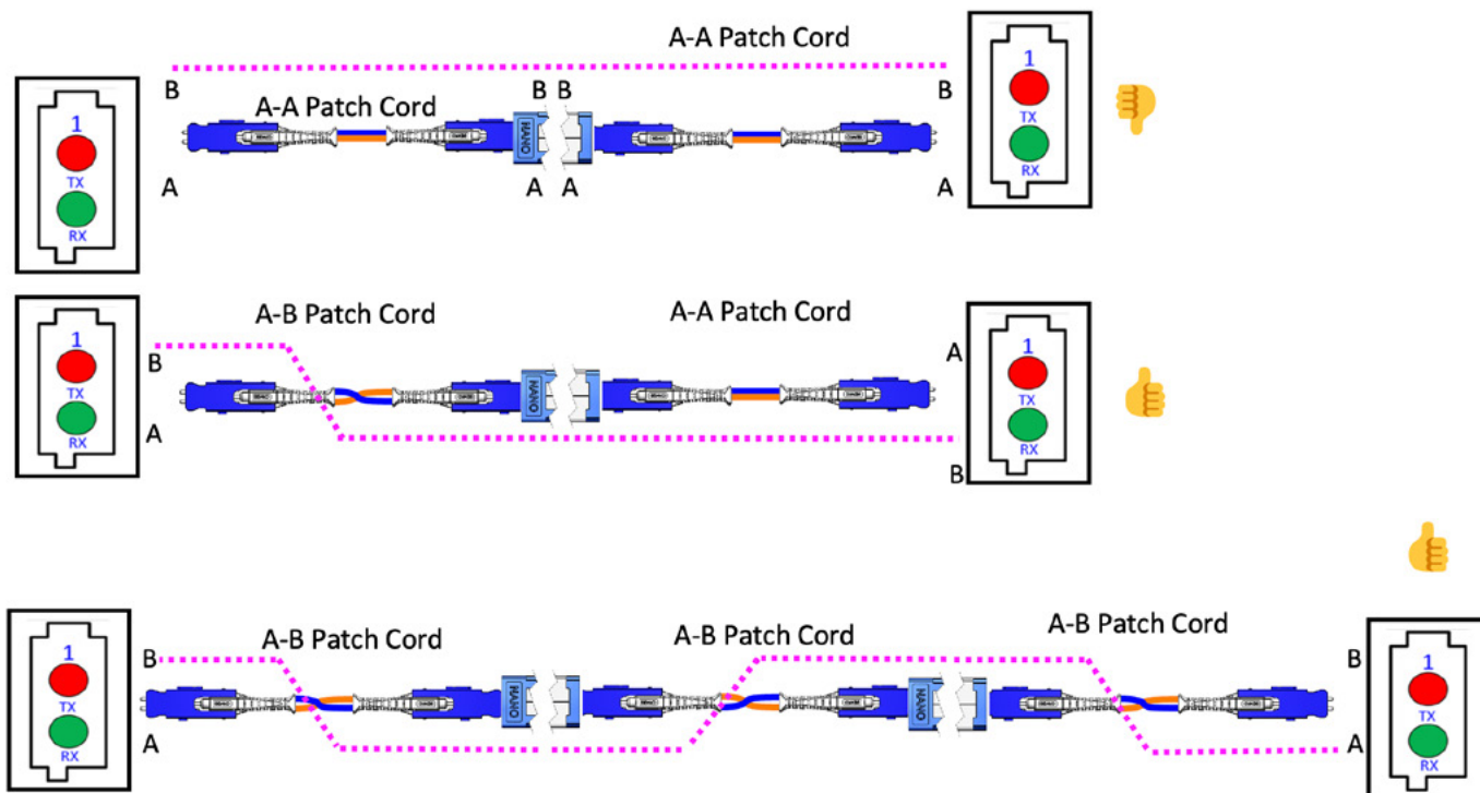
Figure 28 SN® connectors with Key up to Key up adapters must have an odd the number of A-B patchcords
