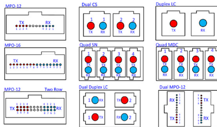
Figure 20 QSFP-DD transceivers active ports configuration
