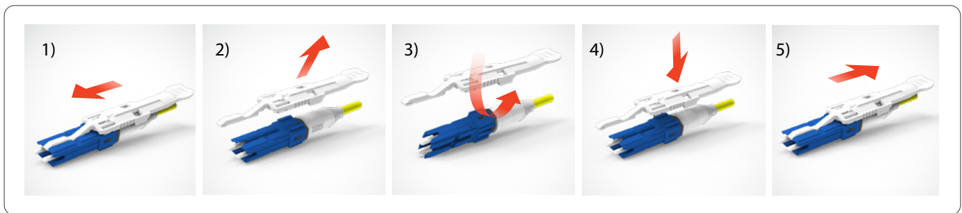
Figure 23 SENKO's CS® EZ-Flip polarity reversal steps
