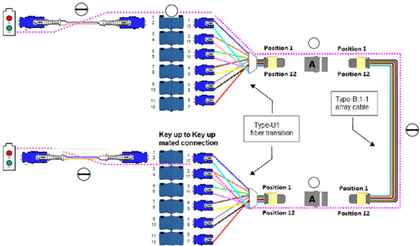
Figure 26 VSFF connectors interconnect with QSFP-DD, cassettes and MPO cables. Method U1 Example.
