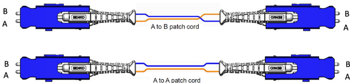
Figure 25 SN® connectors polarity configuration
