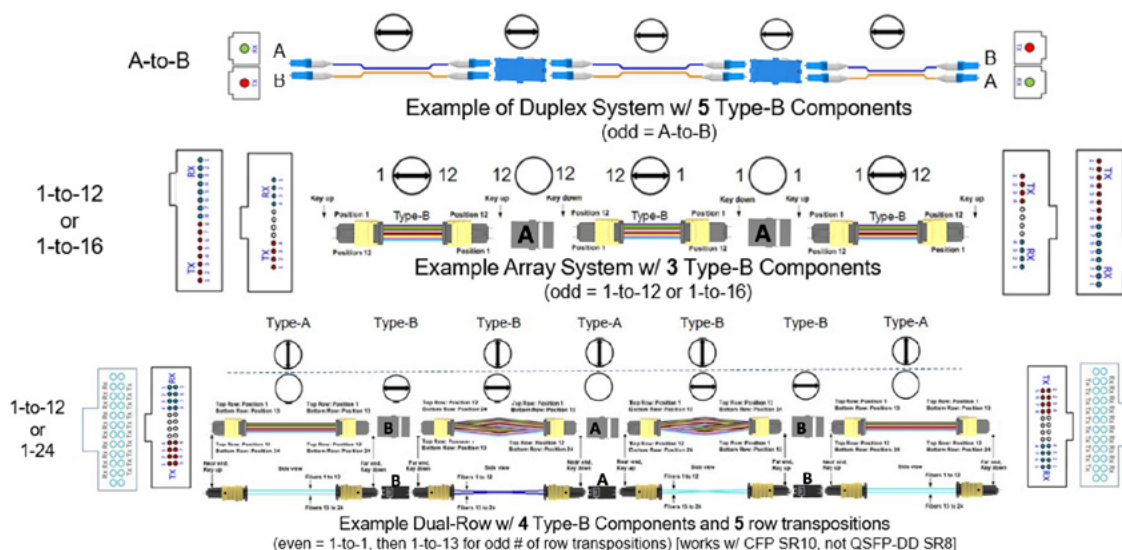
Figure 21 Illustrates how odd number of Type B components transposes the signal
