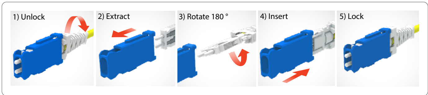
Figure 30 SENKO's SN® EZ-Flip polarity reversal steps
